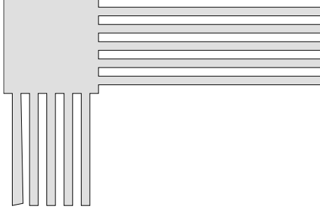
Figure 1: Canonical counterexample
