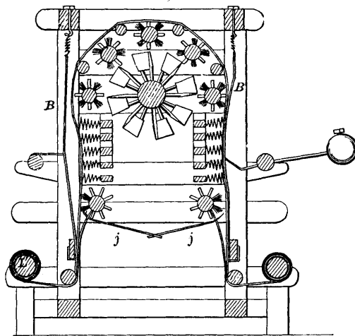
Carpet-Cleaning Machine
