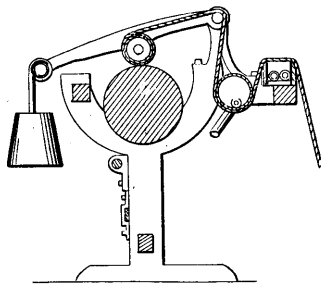
Cloth-Smoothing Machine.
