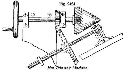
Hat-Printing Machine.
