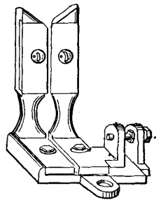
Silk-Cleaning Knife.
