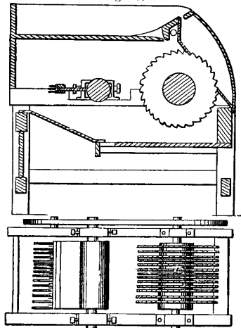
Wool-Picking Machine.
