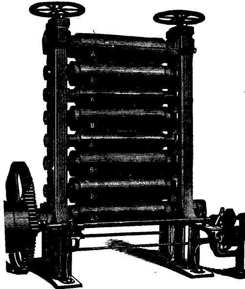
Poole's Super-calender Rolls.
