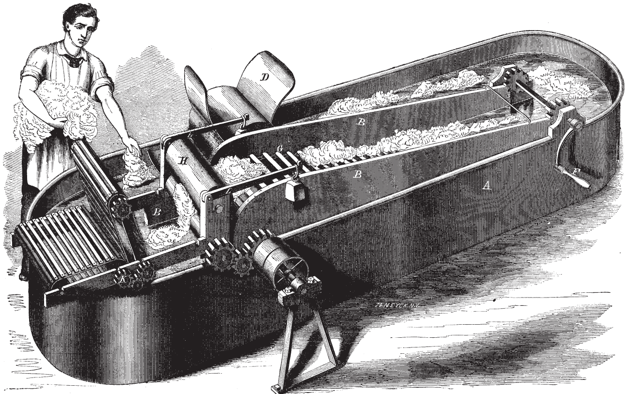
TURNER AND ROBINSON'S WOOL-WASHING APPARATUS.
