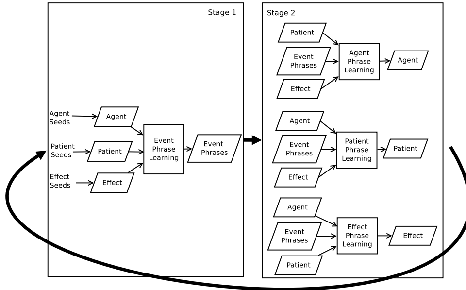
Figure 5.4: Bootstrapped Learning of Event Phrases and Event Facet Phrases for the Terrorism Event Domain.
