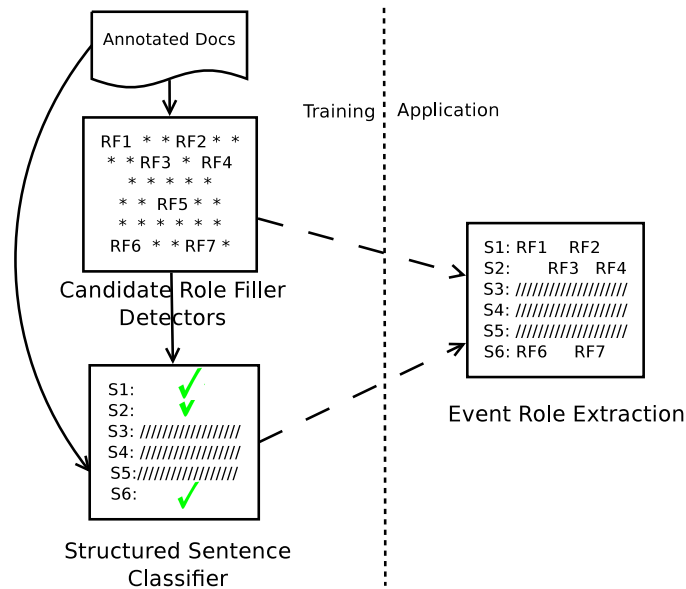
Figure 1.2: LINKER: A Bottom-up Architecture for Event Extraction
