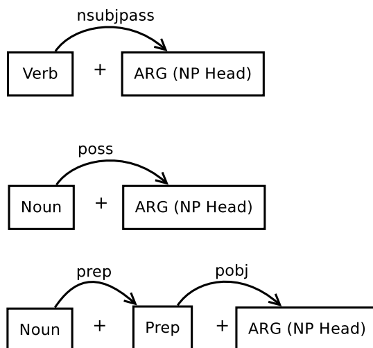
Figure 5.5: Three New Syntactic Structures to Extract Effect Phrases and Patient Terms
