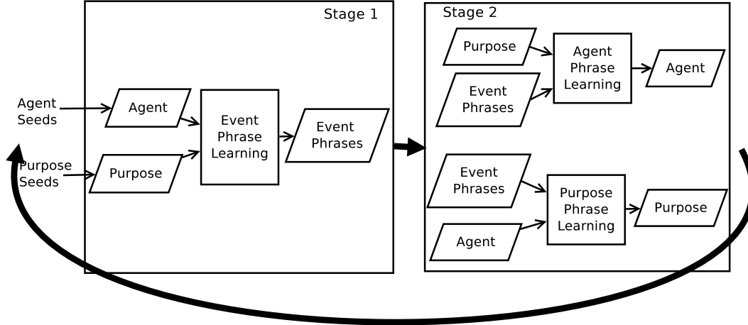
Figure 5.1: Bootstrapped Learning of Event Phrases and Event Facet Phrases for Civil Unrest Event Domain.
