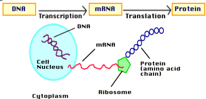
DNA translation.
