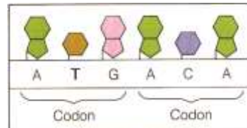
DNA translation.
