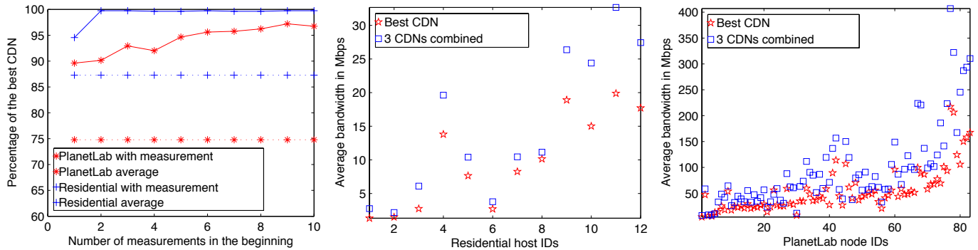
Fig. 19. Measurement based CDN selection: effect of number of measurements Fig. 20. Bandwidth from best CDN vs three combined CDNs for residential hosts Fig. 21. Bandwidth from best CDN vs three combined CDNs for PlanetLab nodes
