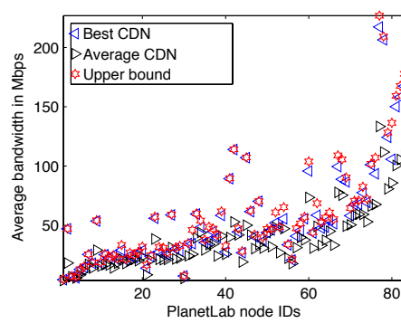
Fig. 18. Average bandwidth for three CDNs and the upper bound at PlanetLab nodes
