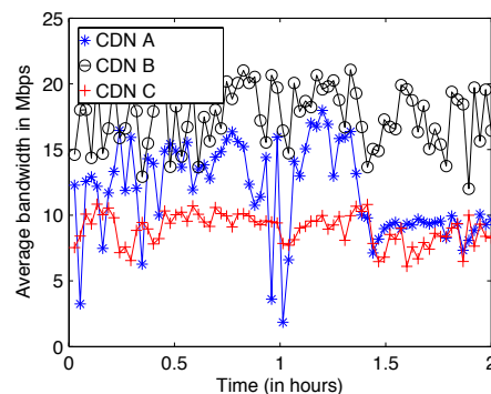
Fig. 15. Instantaneous bandwidth for the three CDNs at residential site 7
