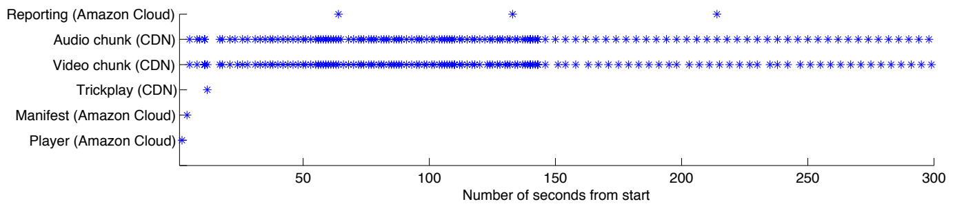
Fig. 2. Timeline in serving a Netflix client
