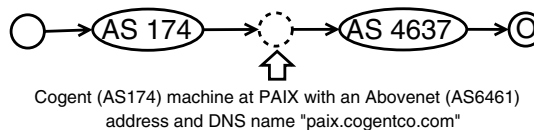
Figure 14: Erroneous AS-level paths due to presence of IXP machines. Here, Next-Hop ASes for O = \{6461, 4637\} , Original AS-level Path = \{ \dots, 174, 6461, 4637, O \} and Rectified AS-level Path = \{ \dots, 174, 4637, O \}
