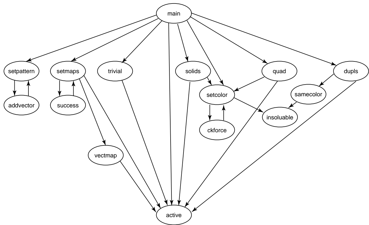
Figure 2. Program Call Graph
