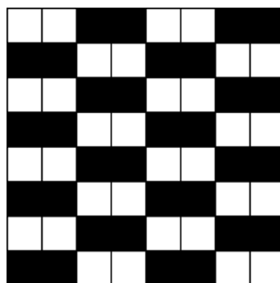
Figure 5. 2/2:2 Tie-Up
