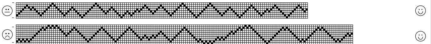
Figure 4. Conservatively Befriended Sequences
