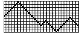
Figure 10. The Befriended Modular-Expanded T-Sequence
