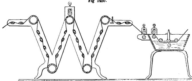
Cord-Drying Machine.
