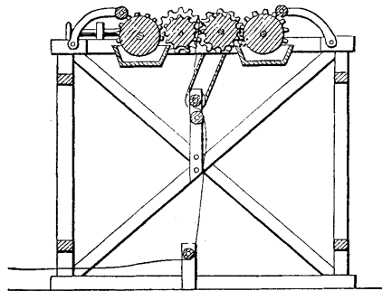
Yarn-Printing Machine.
