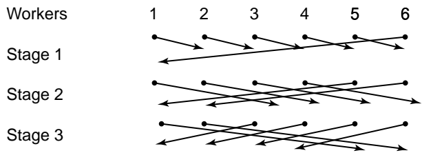
Figure 3.16 Dissemination barrier for 6 processes.
