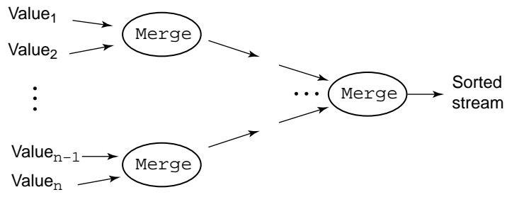
Figure 7.3 A sorting network of Merge processes.
