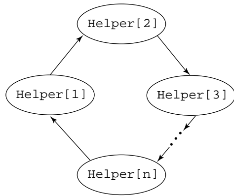
Figure 9.14 A token ring of helper processes.
