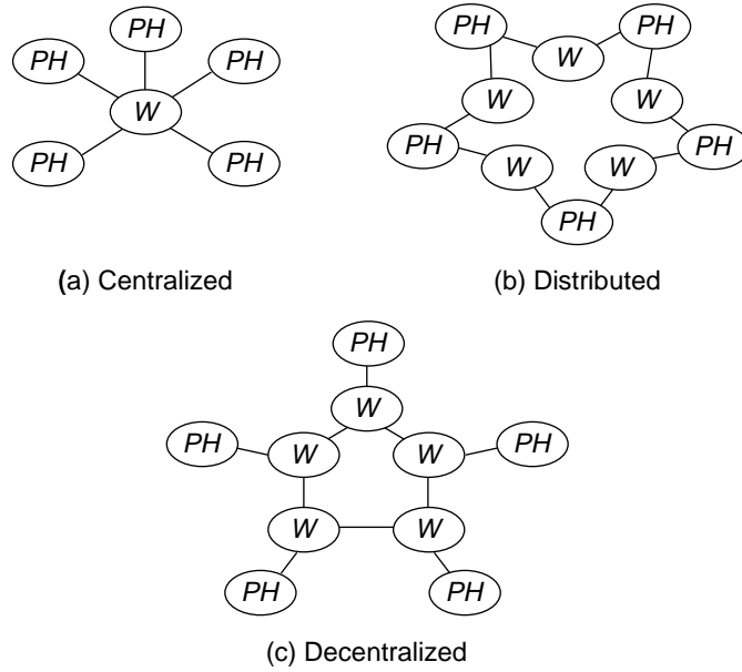
Figure 9.19 Solution structures for the dining philosophers.
