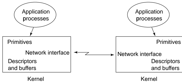
Figure 10.2 Distributed kernel structure and interaction.
