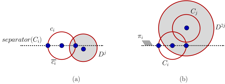
Figure 4: (a) D^j contains an endpoint of c_i (b) center(C_j) \in \pi_i and center(C_i) \in D^{2j} .
