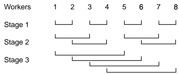
Figure 3.15 Butterfly barrier for 8 processes.
