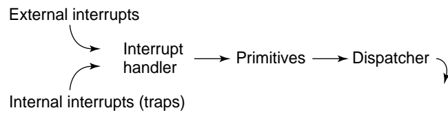
Figure 6.1 Kernel components and flow of control.
