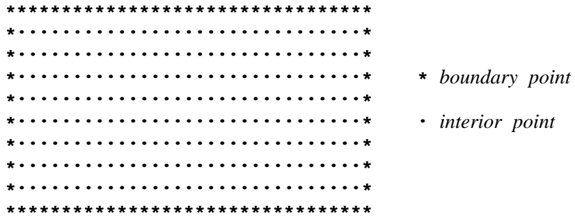
Figure 11.1 Approximating Laplace's equation using a grid.
