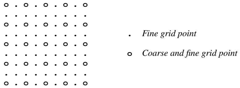
Figure 11.7 Fine and coarse grids, including boundary points.
